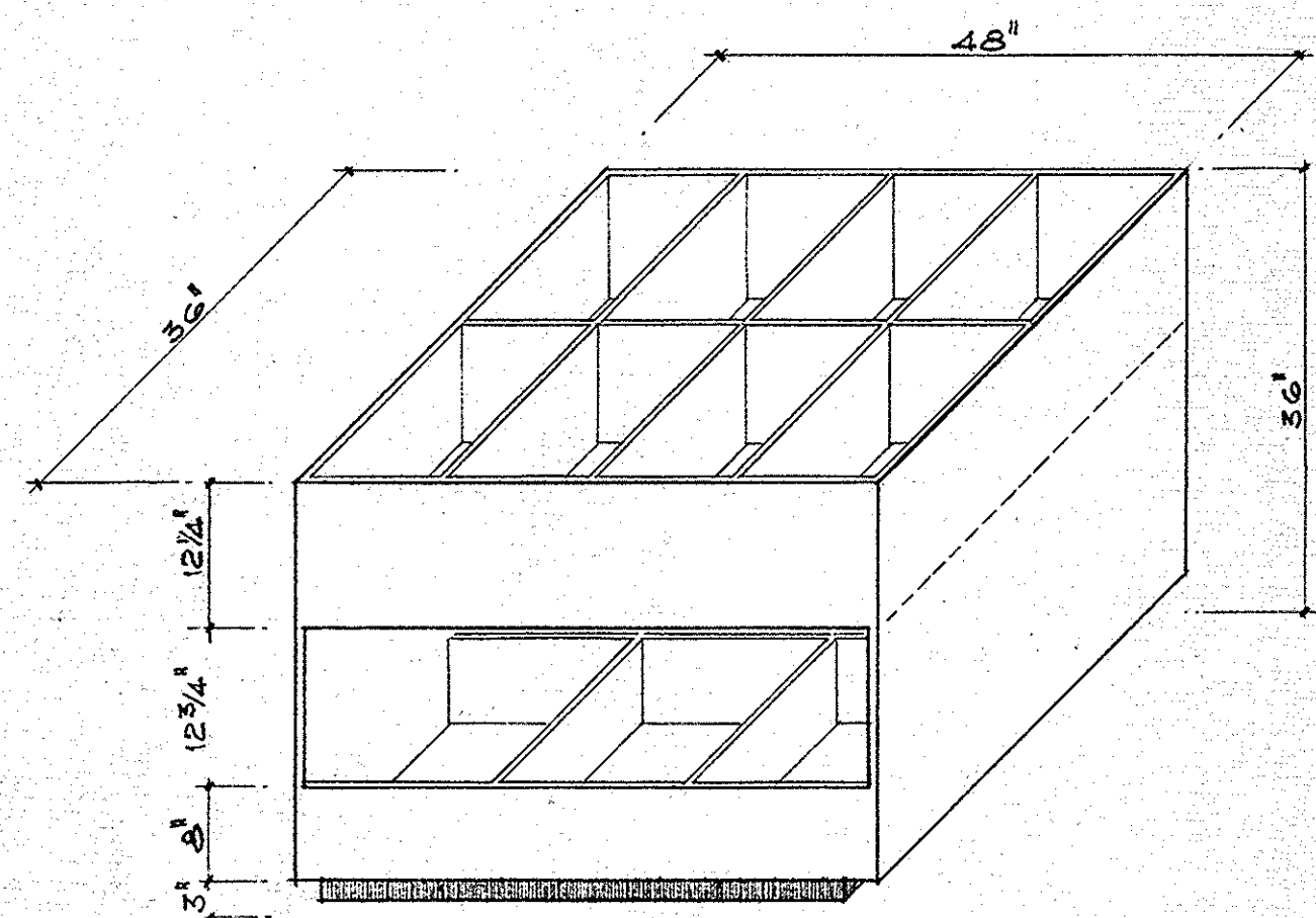
DETAIL ITEM # 13
